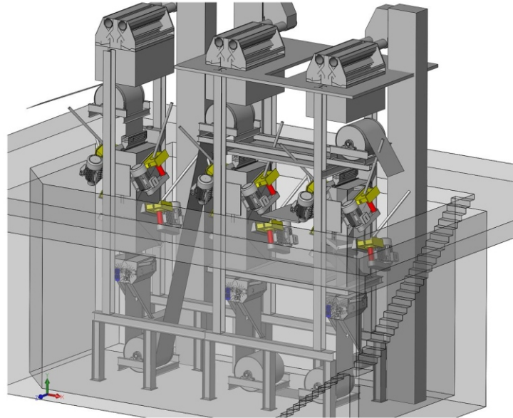
Photo above: 3D picture show a 15m high machine for coil steel strips mechanical cleaning. Slika zgoraj: 3D modelna risba prikazuje 15m visoko postrojenje za mehansko čiščenje trakov.
